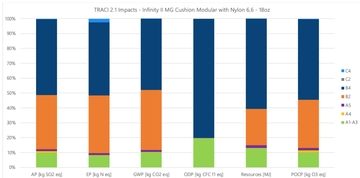
Figure 4: TRACI 2.1 Impacts for Infinity ® 2 MG Cushion Modular with Nylon 6,6 – 18 oz
